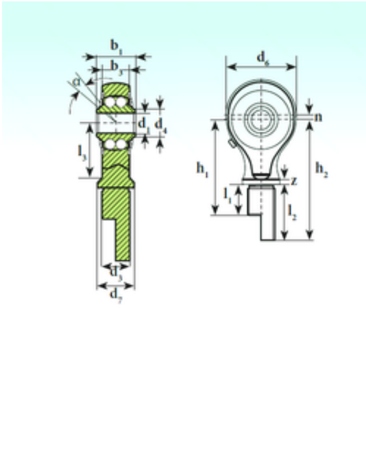
TSM 06-01 BB-E Bearing 2D drawings and 3D CAD models
